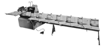
Optional 213 Saddle Extension expands the saddle to six feed stations
