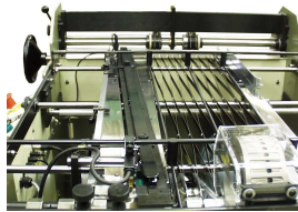
100% accurate registration system including sheet deflectors and micrometer dial for angular adjustments.
